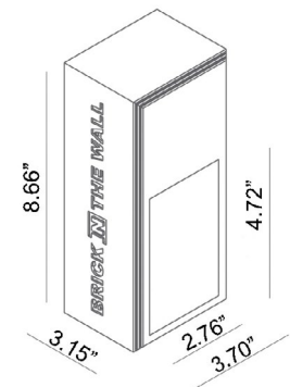
Ceiling Cut-Out: 4.02" x 9.37" Fixture Dimensions
