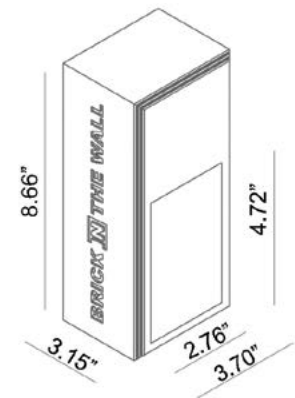
Ceiling Cut-Out: 4.02" x 9.37" Fixture Dimensions
