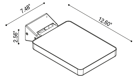
Fixture Dimensions
