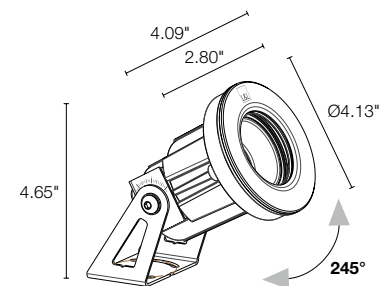
Fixture Dimensions
