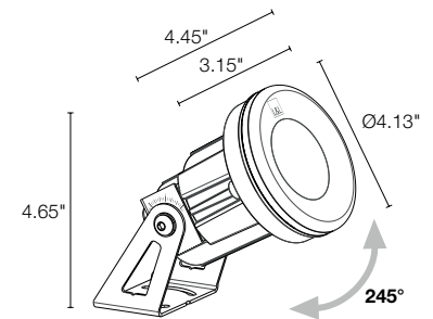
Fixture Dimensions
