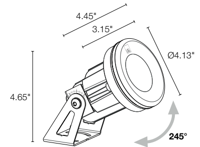
Fixture Dimensions
