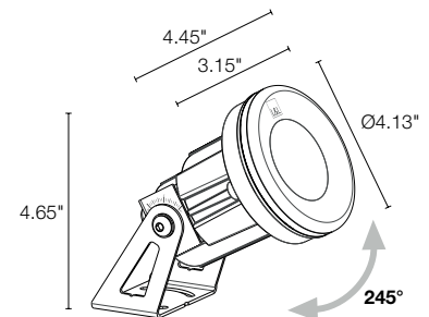
Fixture Dimensions
