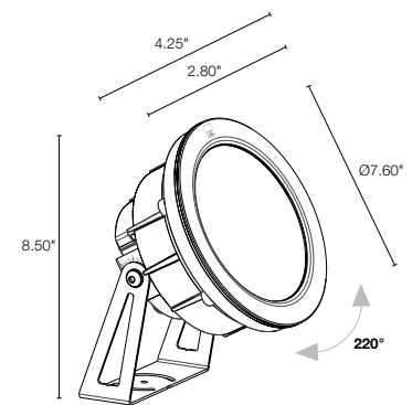
Fixture Dimensions
