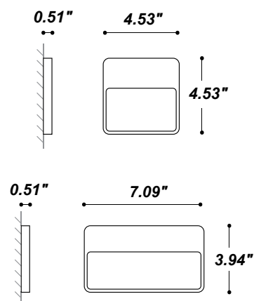
Fixture Dimensions
