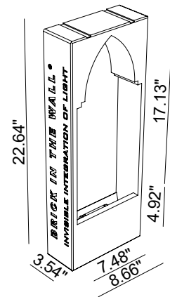
Ceiling Cut-Out: 8.86" x 22.83" Fixture Dimensions
