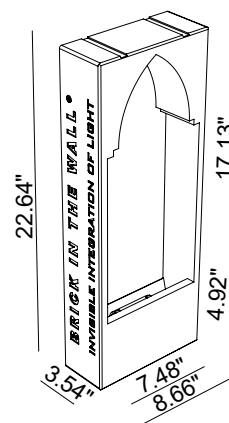
Ceiling Cut-Out: 8.86" x 22.83" Fixture Dimensions
