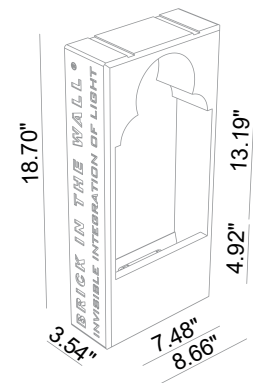
Ceiling Cut-Out: 8.86" x 18.90" Fixture Dimensions
