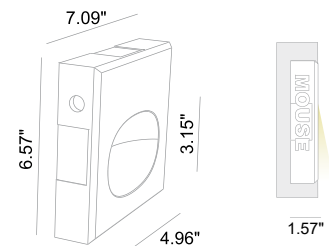
Ceiling Cut-Out: 7.28" x 6.77" Fixture Dimensions
