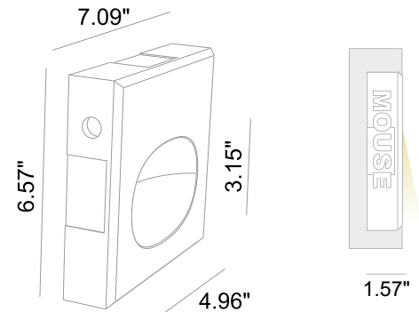
Ceiling Cut-Out: 7.28" x 6.77" Fixture Dimensions
