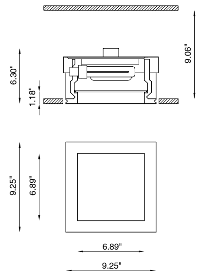
Fixture Dimensions
