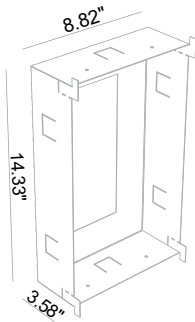
705 01 000 Outer Casing
