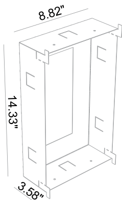
705 01 000 Outer Casing
