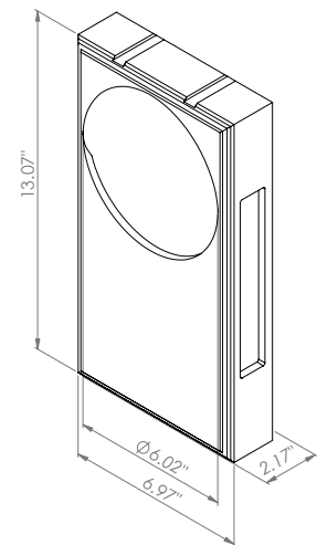
Wall Cut-Out: 7.17" x 13.27" Fixture Dimensions
