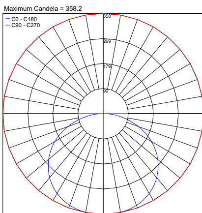
PHOTOMETRIC FILENAME : P2-E LM30.104667.00.DP.BP.20 L78.7IN.IES
