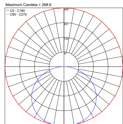
PHOTOMETRIC FILENAME : P2-E LM30.104667.00.DP.BP.20 L59.1IN.IES
