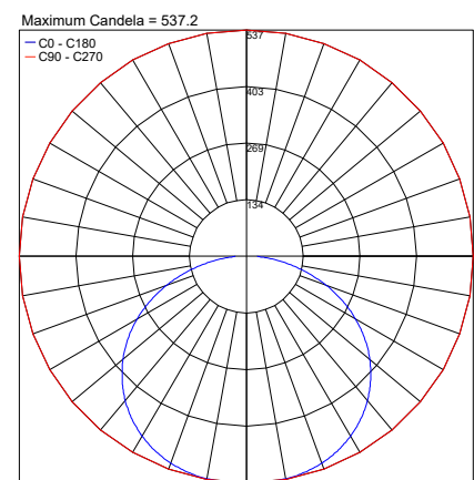
PHOTOMETRIC FILENAME : P2-E LM30.104667.00.DP.BP.20 L118.1IN.IES
