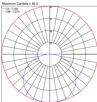
PHOTOMETRIC FILENAME : P2-E LM30.104667.00.DP.BP.20 L19.7IN.IES
