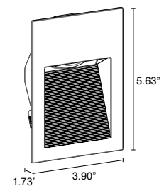
Fixture Dimensions
