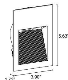
Fixture Dimensions
