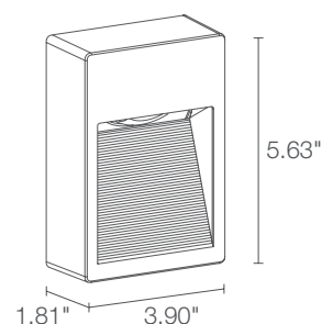
Fixture Dimensions
