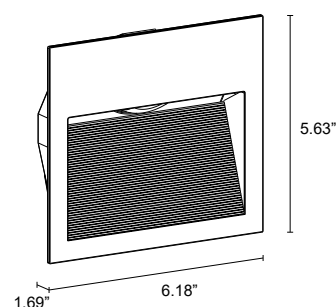
Wall Cut-Out: 5.63" l x 4.92" h Fixture Dimensions
