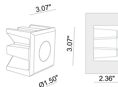
Wall Cut-Out: 3.35" x 3.35" Fixture Dimensions
