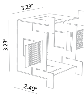
724 01 000 Outer Casing
