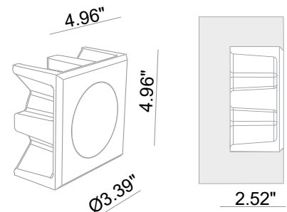
Wall Cut-Out: 5.20" x 5.20" Fixture Dimensions
