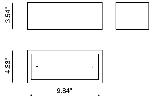
Fixture Dimensions
