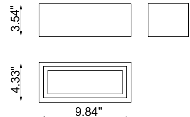
Fixture Dimensions
