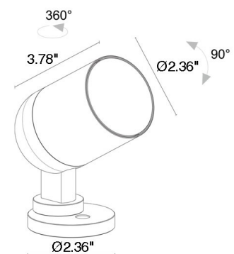
Fixture Dimensions
