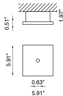
Fixture Dimensions
