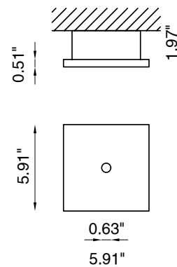
Fixture Dimensions
