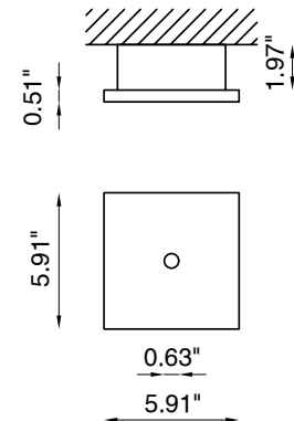
Fixture Dimensions
