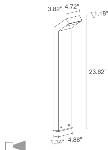
Fixture Dimensions
