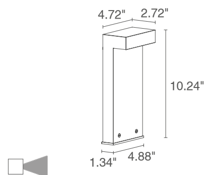
Fixture Dimensions
