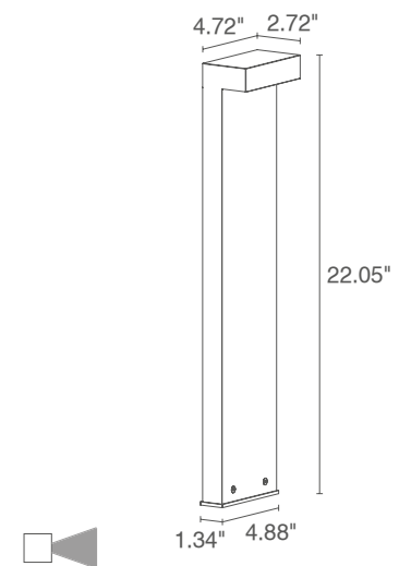
Fixture Dimensions
