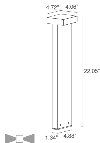
Fixture Dimensions
