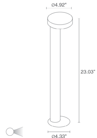
Fixture Dimensions
