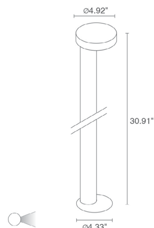
Fixture Dimensions
