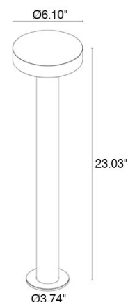
Fixture Dimensions
