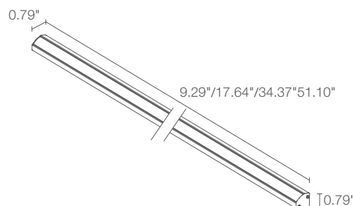
Fixture Dimensions
