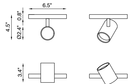
Fixture Dimensions
