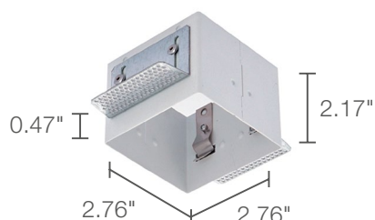
WC2201 Outer Casing ( REQUIRED ) For plasterboard
