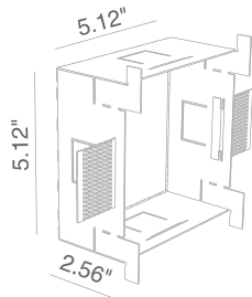
725 01 000 Outer Casing
