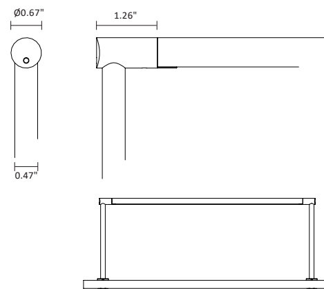
Fixture Dimensions
