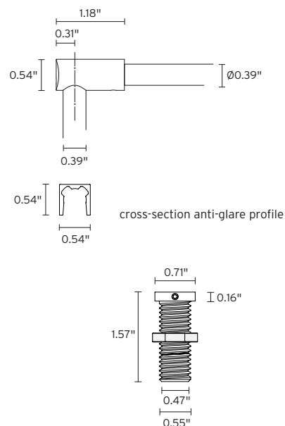
Fixture Dimensions
