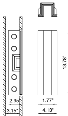
BU6961.AC.US Modular Body 13.78" for each module installed x 4.53" (cut out dimensions)
