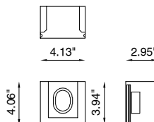
BU6962.AC.US Closure Headparts 4.53" x 4.53" (cut out dimensions)
