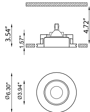
Fixture Dimensions
