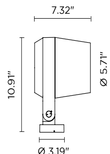
Fixture Dimensions
