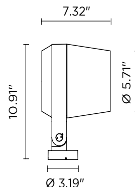
Fixture Dimensions
