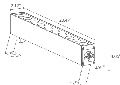
Fixture Dimensions
